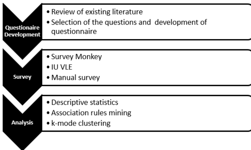
Figure 1 Proposed methodology
